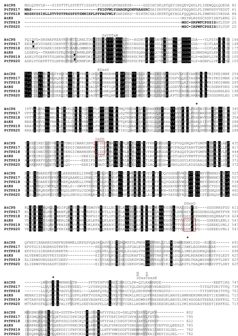
Fig. 2 Amino acid sequence comparison of putative CPS and KS(L) from P. trichocarpa with characterized entCPS and KS from A. thaliana . Identical amino acids are marked by black boxes and amino acids with similar side chains are marked by gray boxes. Conserved motifs are labeled and the highly conserved DxDD and DxxDD motifs are boxed red. Asterisks indicate amino acids important for regulation and product specificity. Predicted N-terminal signal peptides are bold and an arrow indicates the truncation site for heterologous expression. AtCPS (Q38802), ent -copalyl diphosphate synthase; AtKS (Q95AK2), kaurene synthase of Arabidopsis thaliana
