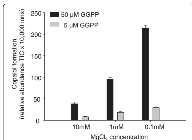
Fig. 4 Sensitivity of PtTPS17 ent -CPP formation to Mg 2+ . The enzyme was expressed in E. coli , extracted, partially purified, and incubated with the substrate GGPP. The product CPP was hydrolyzed using HCl and extracted with hexane and analyzed by GC-MS
