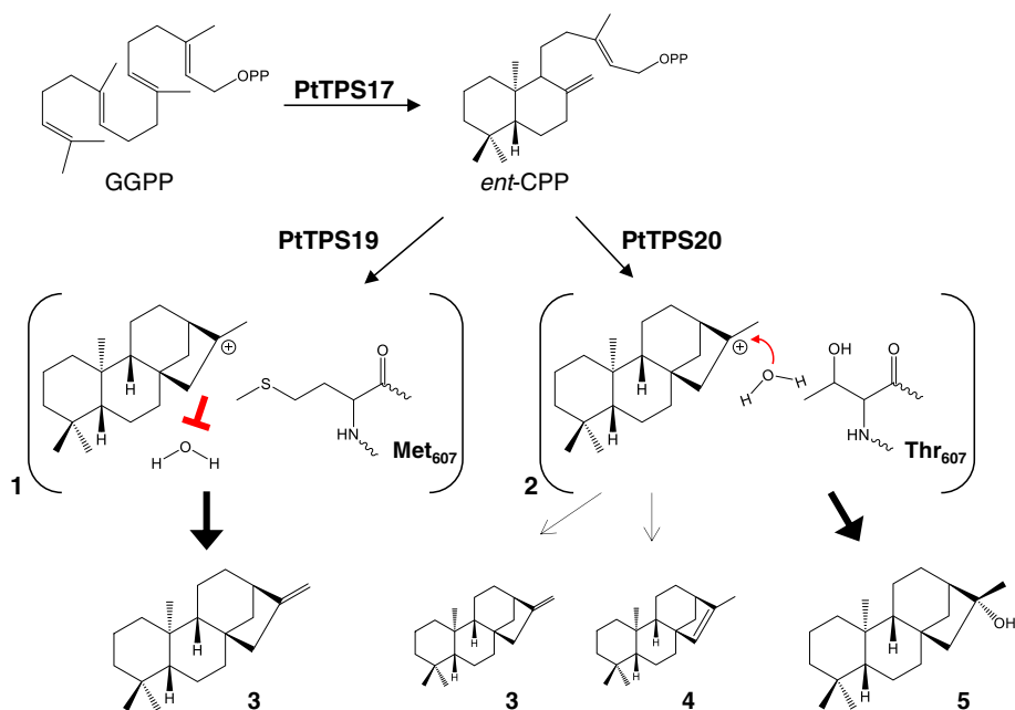
Fig. 8 Putative reaction mechanism for ent -kaurane and 16 \alpha -hydroxy- ent -kaurane formation in poplar. The class II terpene synthase PtTSP17 catalyzes the conversion of GGPP into ent -CPP. Two highly similar class I enzymes, PtTSP19 and PtTSP20 , accept ent -CPP as a substrate and convert it into ent -kaur-16-ene, the precursor for gibberellin biosynthesis or 16 \alpha -hydroxy- ent -kaurane, respectively. The product specificity seems to be controlled by one amino acid in the protein active center excluding (1) or allowing (2) the quenching of the beyeran-16-yl cation by a water molecule (modified from [33]). 3, ent -kaurane; 4, ent -isokaurane; 5, 16 \alpha -hydroxy- ent -kaurane
