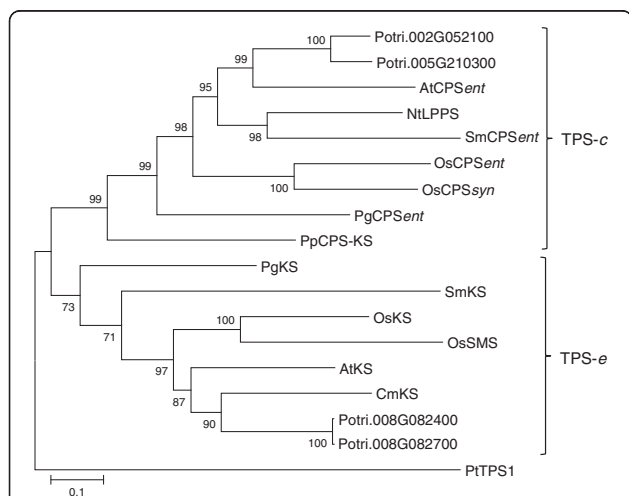
Fig. 1 Phylogenetic tree of putative kaurene synthase-like enzymes (KS(L)) and copalyl diphosphate synthases (CPS). The phylogenetic relationship of putative KS(L) and CPS synthases from P. trichocarpa to KS(L) and CPS from other plant species is shown. The tree was inferred with the neighbor-joining method and n = 1000 replicates for bootstrapping. Bootstrap values are shown next to each node. TPS- c and TPS- e , represent established TPS subfamilies [13]. PtTPS1 was used as an outgroup. KS: ent -kaur-16-ene synthase, SMS: stemar-13-ene synthase, LPPS: 8-hydroxy-copalyl diphosphate synthase, CPS: copalyl diphosphate synthase, Nt: Nicotiana tabacum , Cm: Cucurbita maxima , At: Arabidopsis thaliana , Os: Oryza sativa , Pg: Picea glauca , Potri: Populus trichocarpa , Sm: Salvia miltiorrhiza , Pp: Physcomitrella patens
