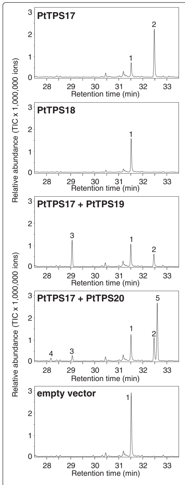
Fig. 3 GC-MS analysis of diterpenoids produced by recombinant PtTPS17, PtTPS18, PtTPS19 and PtTPS20. The enzymes were expressed in E. coli , extracted, partially purified, and incubated with the substrate GGPP. Products were extracted with hexane and analyzed by GC-MS. 1, geranylinalool; 2, copalol; 3, ent -kaurene; 4, ent -isokaurene; 5, 16 \alpha -hydroxy- ent -kaurane
