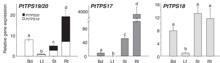
Fig. 6 Transcript abundance of PtTSP19/20 , PtTSP17 and PtTSP18 genes in different organs of P. trichocarpa . Gene expression in leaf buds (Bd), leaves (Lf), stem (St) and roots (Rt) was measured using qRT-PCR. PtTSP19 to PtTSP20 ratio was determined through repeated sequencing of amplicons. Means and standard errors are shown ( n = 6 ). A one way ANOVA followed by a Holm-Sidak test was used to test for statistical significance. Different letters indicate significant differences between plant organs. PtTSP19/20 : F = 140.549 , p < 0.001 ; PtTSP17 : F = 271.955 , p < 0.001 ; PtTSP18 : F = 31.952 , p < 0.001
