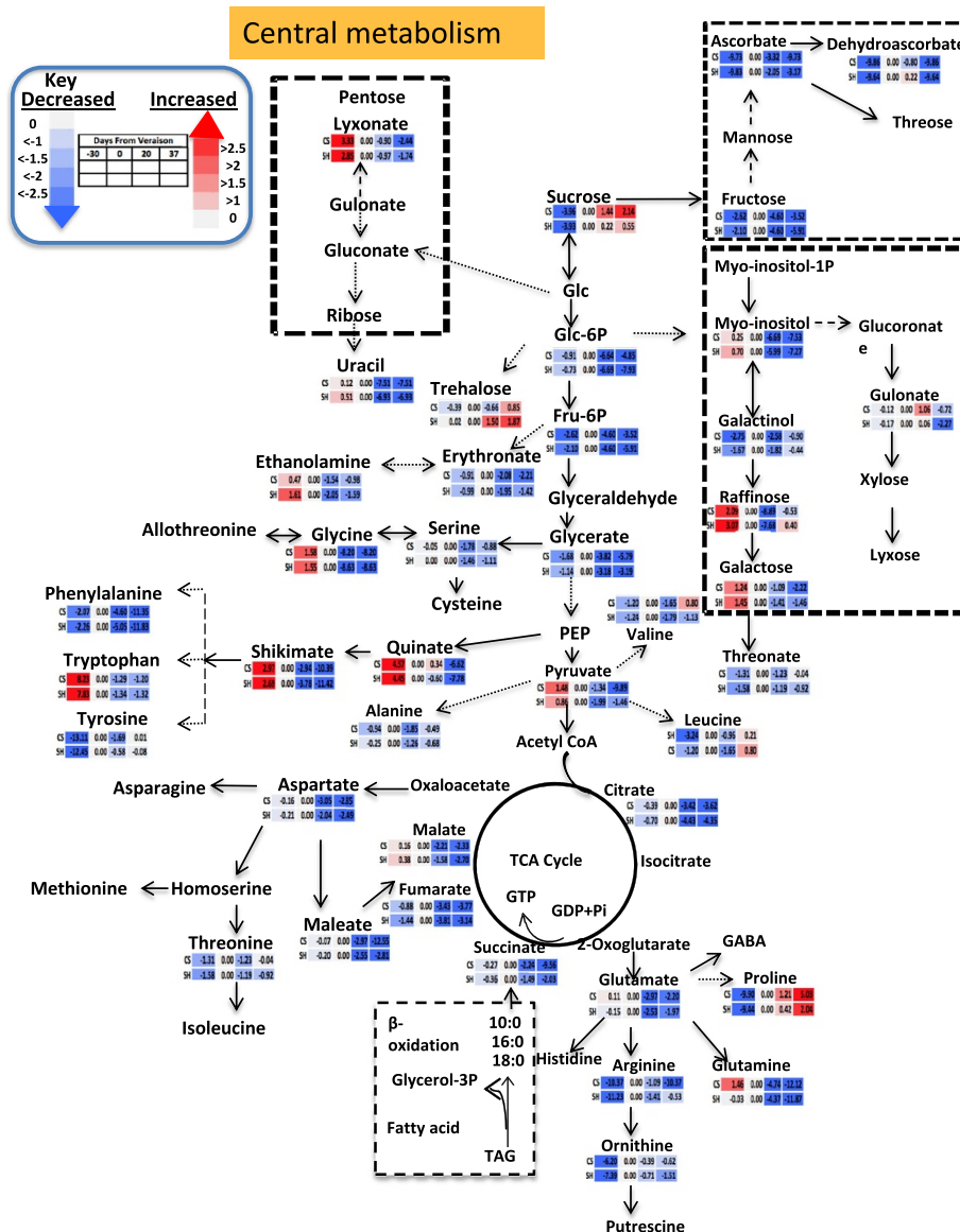
Figure 3 Schematic representation of primary metabolite pathways with log 2 transformed fold change normalized to the veraison stage of each cultivar. Different colors represent the increase (red) or decrease (blue) of the metabolites fold change as indicated in the color index. n = 6. Each row (upper row CS and lower row Shiraz) metabolite change with reference to veraison stage, where as each column represents different time points (the diagram was generated by using pathway tool program [84]).
