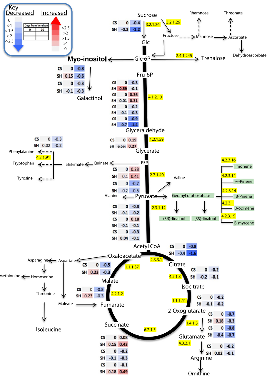
Figure 6 Berry skin transcripts involved in the primary metabolism and changing significantly from veraison to post veraison stage in Shiraz and CS. The data were normalized to the respective transcript abundance in CS veraison stage. Heatmaps represent changes in transcript expression levels ( \log_2 transformed) as indicated by the color legend and by the values within each box. EC numbers for the mentioned enzymes are: 3.2.1.26 (Fructofuranosidase), 2.4.1.245 (Trehalose synthase), 4.1.2.13 (Fructose-bisphosphate aldolase), 2.7.1.40 (Pyruvate kinase), 1.2.1.59 (Glyceraldehyde-3-phosphate dehydrogenase), 2.7.1.40 (Pyruvate kinase), 2.3.1.12 (Acyl-CoA:dolichol acyltransferase), 4.2.3.16 (Limonene synthase), 4.2.3.14 (Pinene synthase), 4.2.3.15 (Myrcene synthase), 2.3.3.1 (Citrate (Si)-synthase), 4.2.1.3 (Aconitase), 1.1.1.41 (Isocitrate dehydrogenase), 1.4.1.3 (Glutamate dehydrogenase), 4.3.2.1 (Argininosuccinate lyase), 4.2.1.5 (Arabinonate dehydratase), 6.2.1.5 (Succinyl-CoA synthetase), 4.2.1.2 (Fumarate hydratase), 1.1.1.37 (Malate dehydrogenase) 4.2.1.91 (Arogenate dehydratase) (the diagram was generated by using pathway tool program [84]).
