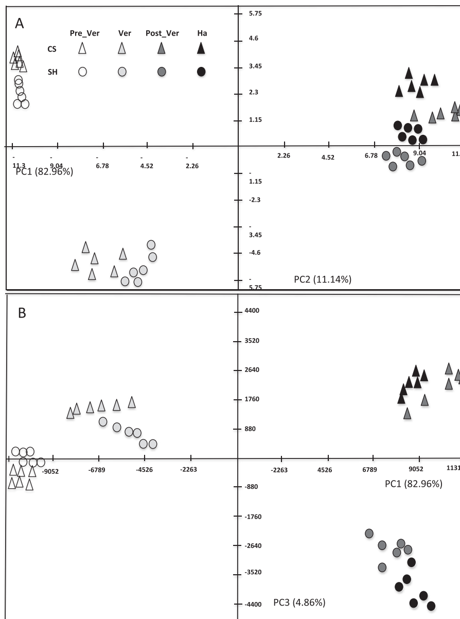
Figure 4 Metabolic shift of specialized metabolism during berry development in Cabernet Sauvignon and Shiraz. PCA plot of PC1 versus PC2 (A) and PC1 versus PC3 (B) of metabolite profiles of Cabernet Sauvignon and Shiraz at four berry development stages. Percentage of the variance captured by each PC is given close to each respective axis. Each point in (A) and (B) represents one biological sample.
