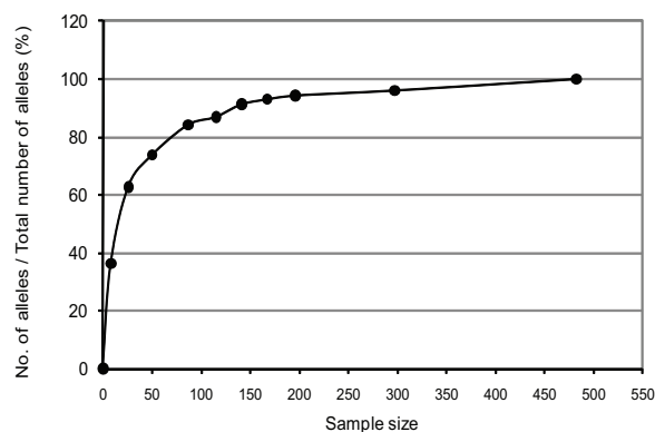
Figure 1 Relationship between the percentage of alleles retained from the thematic collection and the sample size of thematic core collections.
