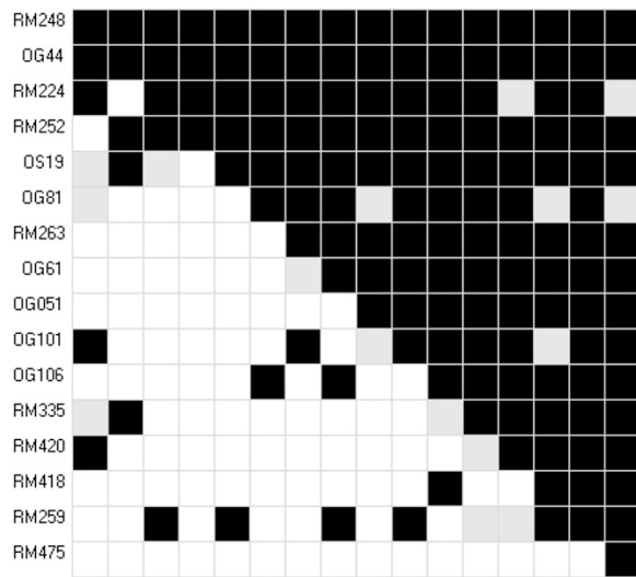
Figure 2 Sampling effect in measurements of linkage disequilibrium between 16 microsatellite loci. Sampling effect in measurements of linkage disequilibrium between 16 microsatellite loci. The upper triangle represents values of significance for the 485 accessions of the thematic collection; the lower triangle represents values of significance for the thematic core collection of 87 accessions (CC Corex ). Black boxes indicate high significance ( p < 0.0001 ); gray boxes indicate intermediate values ( 0.01 > p > 0.0001 ); white boxes indicate low levels of significance ( p > 0.01 ).
