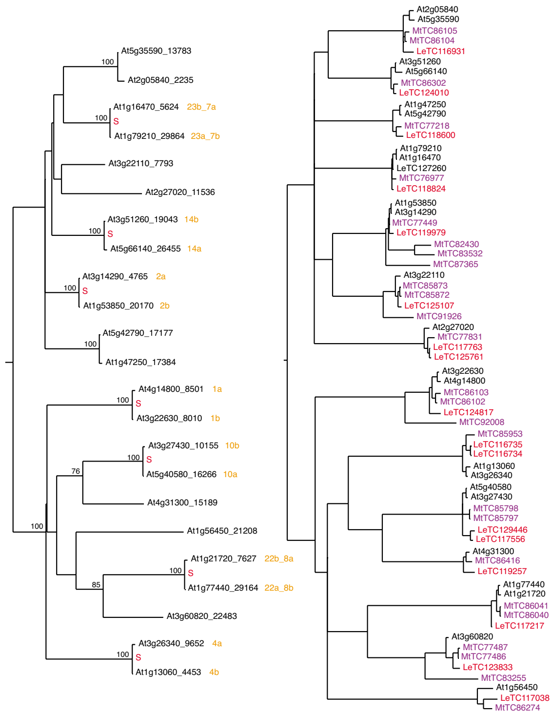
Figure 5 Proteasome 20S subunit family: low tandem, high segmental The phylogeny on the left shows segmental duplications in the A. thaliana proteasome 20S subunit family, which lacks tandem duplications. The phylogeny on the right represents the same A. thaliana sequences but with M. truncatula and tomato EST sequences added to evaluate the degree to which these homologs are conserved. Relationships of clades represented in both phylogenies are in general agreement, with some differences due to instabilities of some deep nodes.
